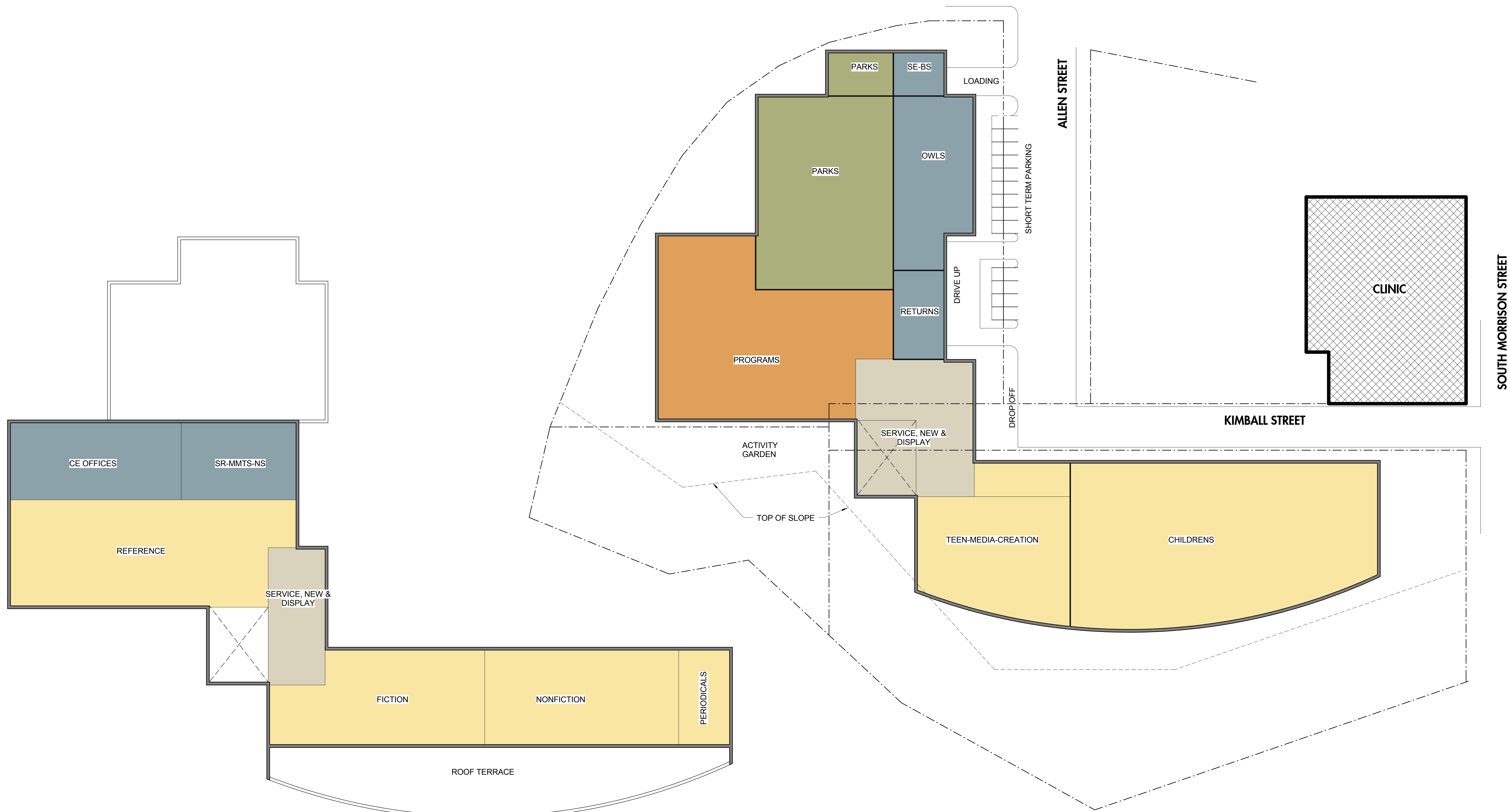
1 Level 1 Design SCALE: 1/32" = 1'-0"
